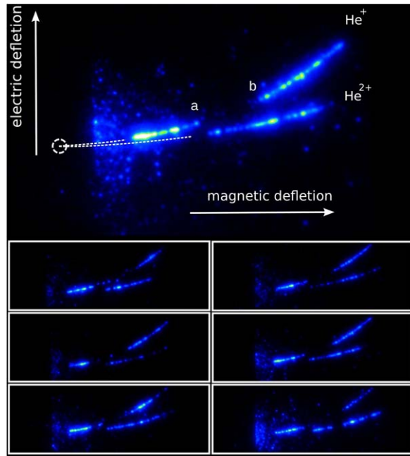
Figure 2. Raw pictures from the Thomson parabola at 80°, with each one corresponding to a single shot for n_e = 2.8 \times 10^{19} \text{ cm}^{-3} with I = 1.3 \times 10^{19} \text{ W cm}^{-2} . The neutral blob (dashed circle) is filtered out and the dotted lines indicate the fit dispersion traces for each species. The dispersive magnetic field reads B = 0.25 \text{ T} . Points a and b are located at 55 and 28 keV in the \text{He}^+ spectrum.
