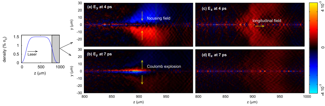
Figure 4. The transverse (left) and longitudinal (right) electric field (in units of a_0 ) in the falling density ramp of the plasma at 4 ps (top) and 7 ps (bottom). The plotted region is indicated in gray in the inset, and shows the density profile of the gas jet. The dashed line roughly indicates the position of the interface plasma/vacuum.
